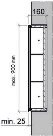
MIRR 6 EINBAU | for installation in the niche
